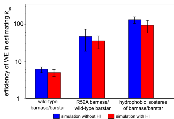
Figure 4. Average efficiencies of WE relative to brute force simulation in computing the k_{on} . Full details for estimating efficiencies are described in Methods . Uncertainties represent 95% confidence intervals for averages from five independent WE simulations.
